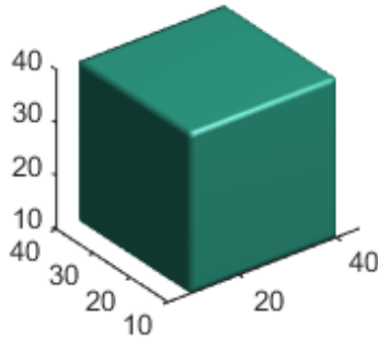
Chessboard
