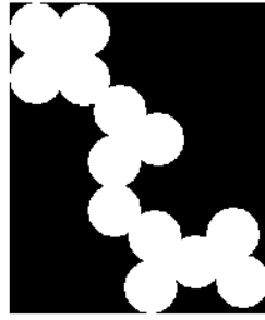
Image Returned
