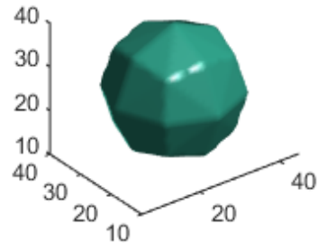
Quasi-Euclidean
